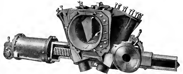
Driving Mechanism of the Duplex Locomotive Stoker Showing the Vance for Distributing the Coal to the Vertical Screws
